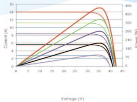
Current-Voltage & Power-Voltage Curves (430W)
